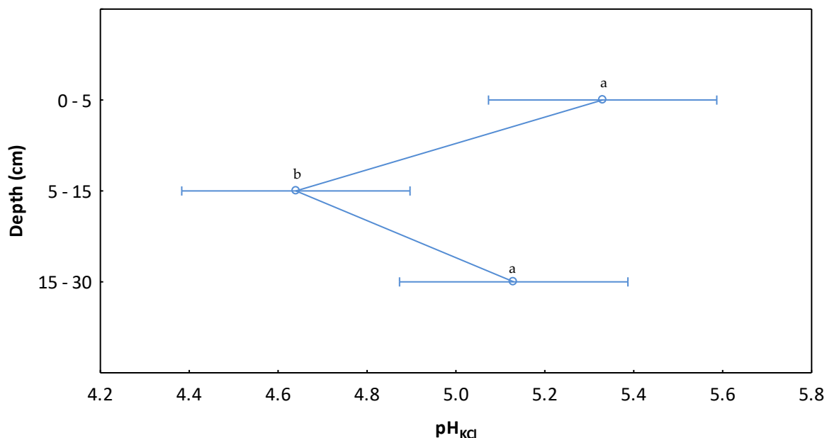
Figure 3.3. Stratification of pH KCl between 0 – 5, 5 – 15, and 15 – 30 cm soil depth of soils with at least one depth increment with pH KCl ≤ 5.0. No common superscript letter indicates a significant ( p \leq 0.05 ) difference.
