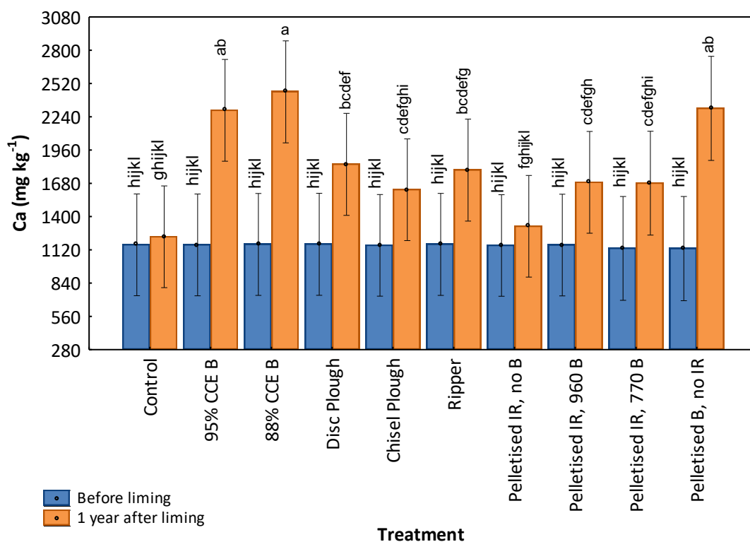
Figure 4.8. The Ca (mg kg -1 ) concentration for all the treatments at the 0 – 5 cm depth before and one year after liming. Common letters indicate no significant difference. B = Broadcast, CCE = Calcium carbonate equivalent, IR = In-row placement.
