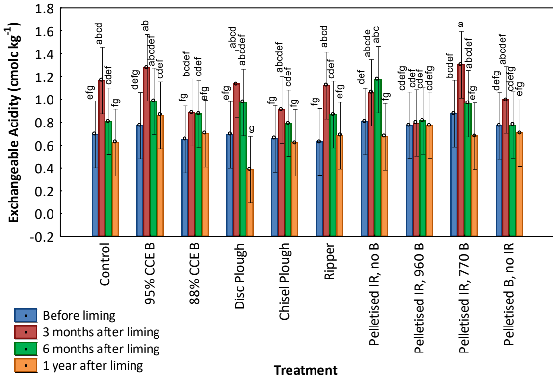
Figure 4.16. The exchangeable acidity ( \text{cmolc kg}^{-1} ) of the treatments over time at the 5 – 15 cm depth. Common letters indicate no significant difference. B = Broadcast, CCE = Calcium carbonate equivalent, IR = In-row placement.
