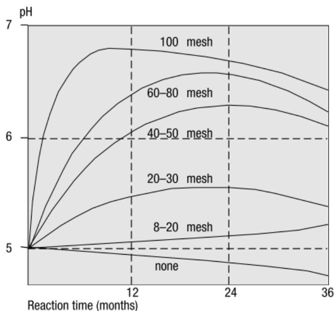
Figure 2.2. The effect of fineness on the speed of lime reaction (an increase in mesh number indicates smaller lime particles). (Beegle, 2001).
