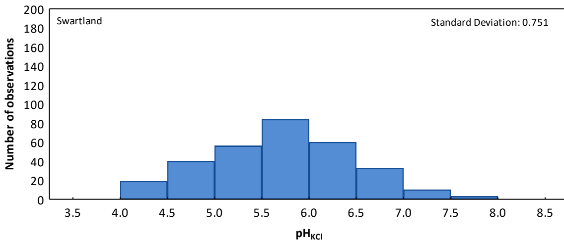
Figure 3.2. The mean soil pH KCl distribution for all samples (top) as well for the southern Cape (middle) and the Swartland (bottom) regions separately.
